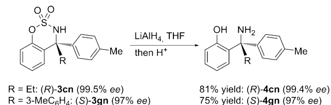
Scheme 2. Ring opening of the asymmetric arylation products 3 .
