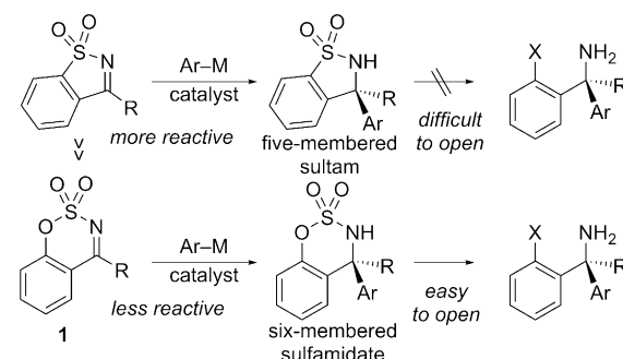
Scheme 1. Reactivity and utility of cyclic N -sulfonyl imines.
